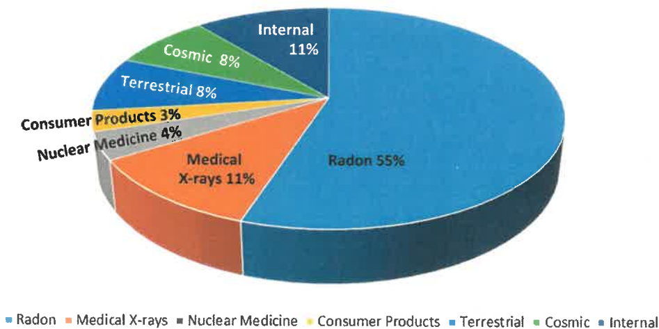
Ionizing Radiation Exposure of the US Population (2006)
